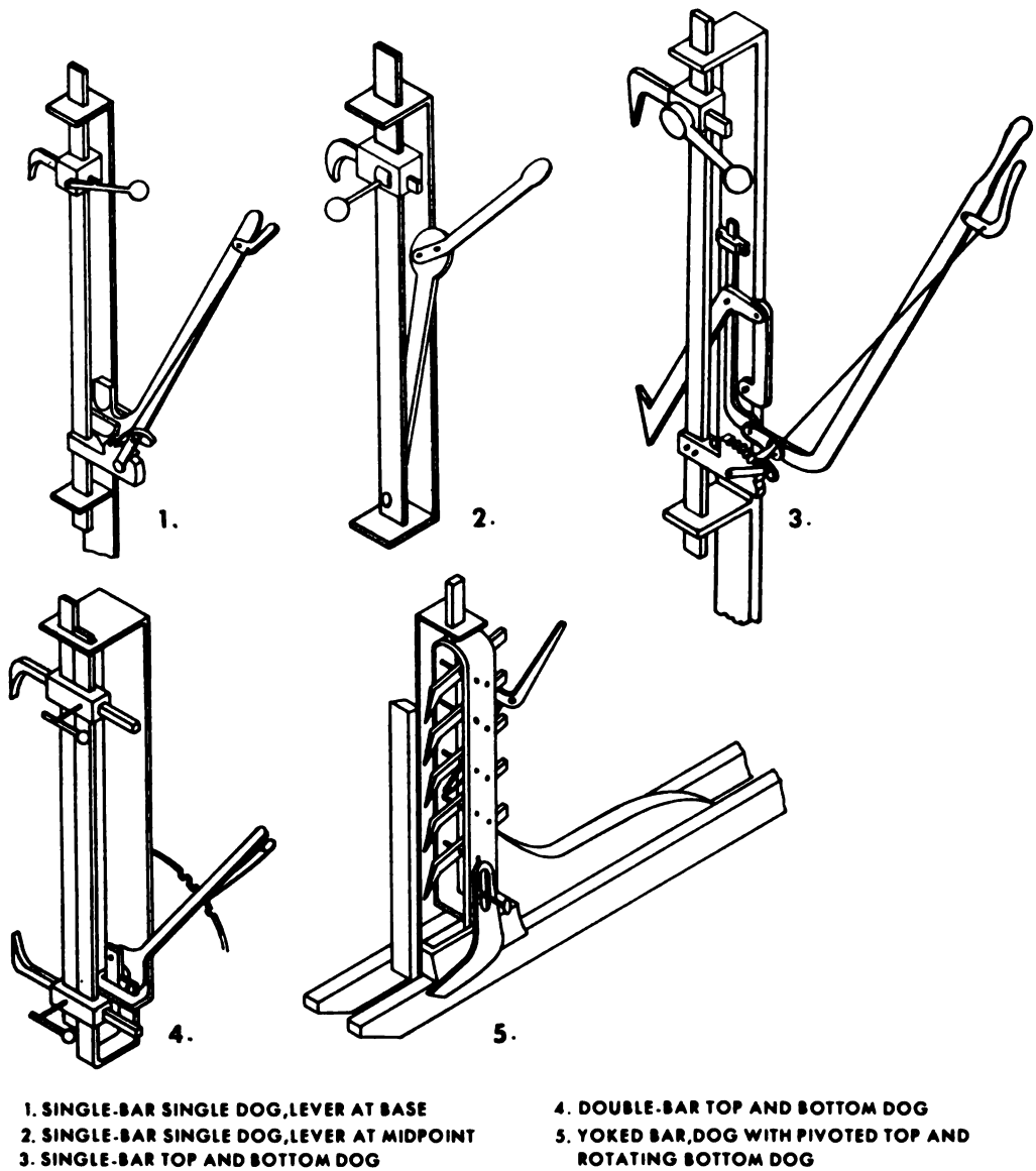
Figure 8-13. Housing-post types of manually operated dog.
